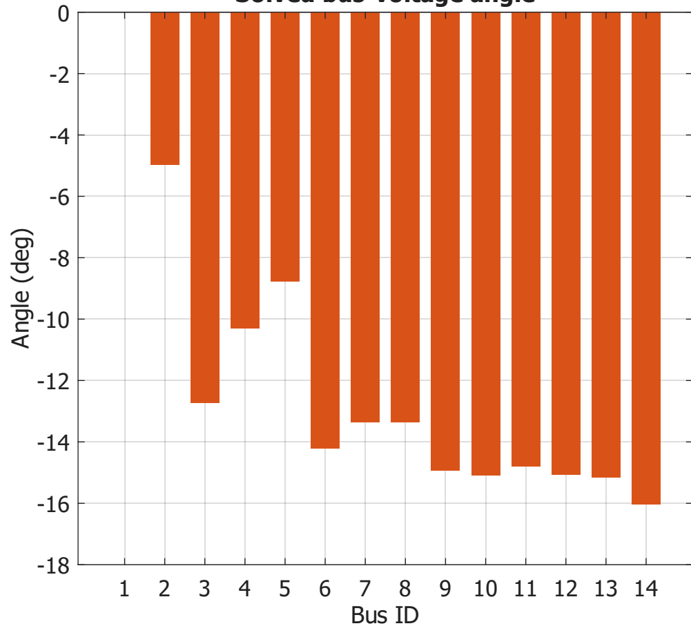
Solved bus-voltage angle
