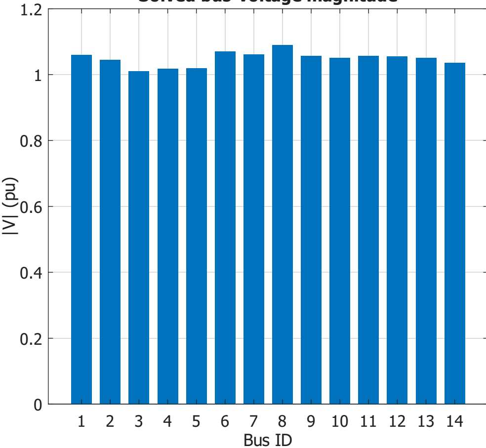
Solved bus-voltage magnitude
