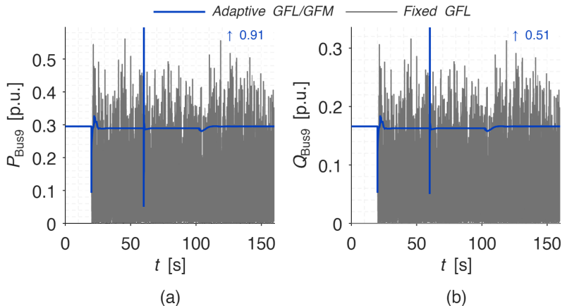
Figure 10: Active and Reactive Power
