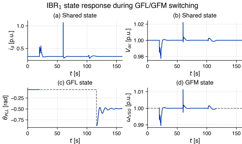
Figure 4: IBR 1 : blue = active; grey dashed = inactive stored state
