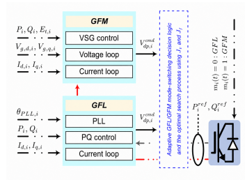
Figure 2: Switchable controller branches.
