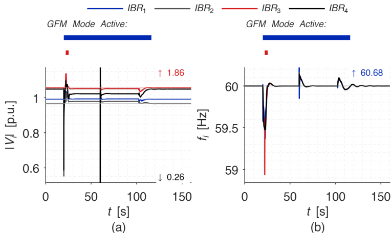
Figure 7: Converter-bus voltage and active-controller frequency
