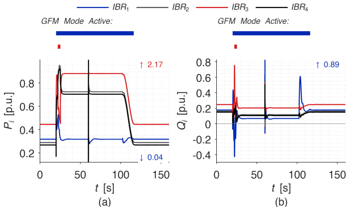
Figure 10: Converter power responses: (a) active power and (b) reactive power.
