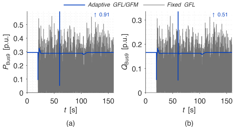
Figure 12: Bus-9 power responses for adaptive GFL/GFM and fixed-GFL cases: (a) active power and (b) reactive power.
