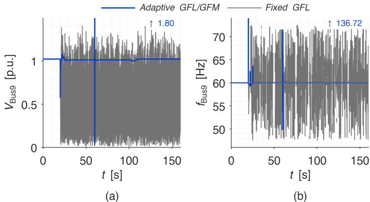
Figure 11: Bus-9 responses for adaptive GFL/GFM and fixed-GFL cases: (a) voltage magnitude and (b) frequency.
