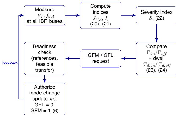
Figure 3: Supervisory readiness and GFL/GFM mode-switching procedure.
