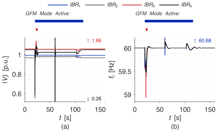
Figure 9: Converter responses: (a) bus-voltage magnitude and (b) converter frequency.
