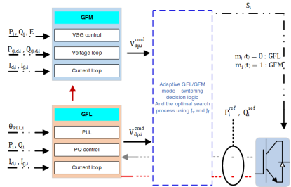
Figure 2: Switchable controller branches.
