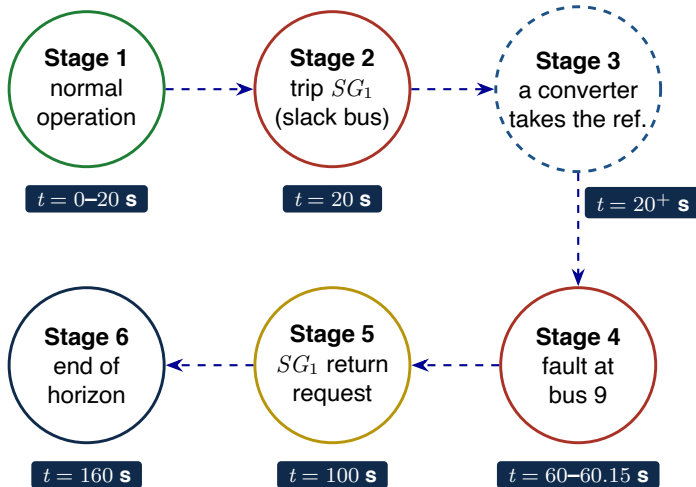
Figure 5: Scenario timeline. Breaker reclose after synchronism: 102.363 s; final IBR return to GFL: 116.238 s.
