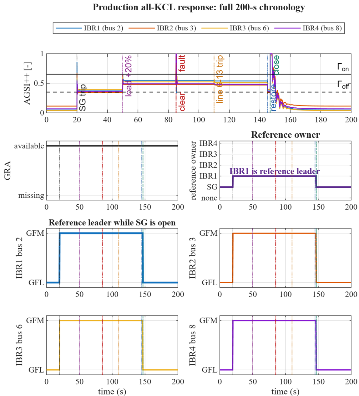
Figure 4: Bounded AGSI++, GRA, reference ownership, and separate IBR1–IBR4 mode time-lines. The owner trace identifies IBR1 at bus 2 as the grid-forming angle/frequency leader while the SG is open. All IBRs are GFL before 20 s, GFM until the accepted handback, and GFL thereafter.
