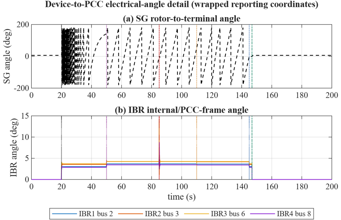
Figure 6: Angle detail. The offline SG rotor slips relative to the energized grid; the plotted coordinate is wrapped to [-180, 180) degrees.
