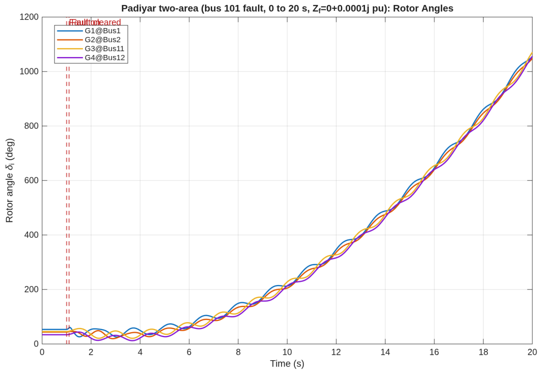
Figure 6: Bus-101 project fault response using the AVR configuration (the book's 20-state model): stored absolute generator rotor angles \delta_i(t) in degrees. No initial-angle subtraction is applied. Red markers identify fault application and clearance. The simulated interval is 0–20 s and Z_f = j10^{-4} pu.
