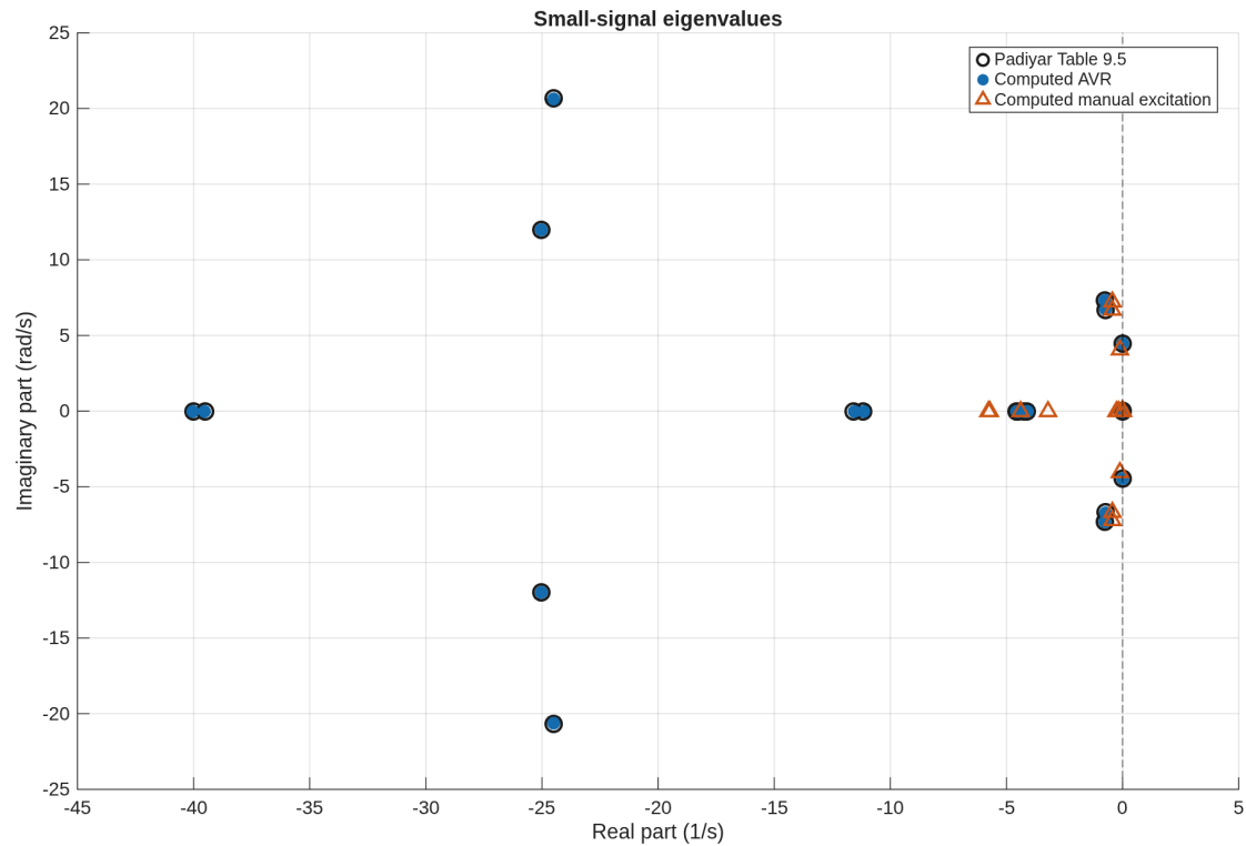
Figure 4: Graphical counterpart of Table 9: the full computed manual/AVR eigenvalue spectrum and the independently transcribed Table 9.5 values.
