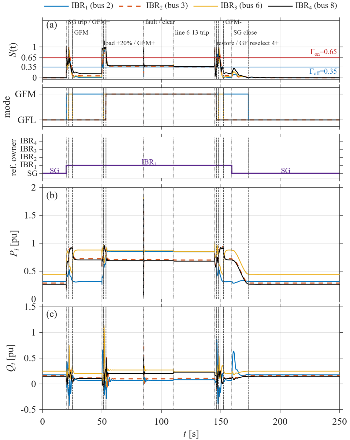
Figure 5: (a) Severity index S per converter with both switching thresholds, \Gamma_{on} = 0.65 and \Gamma_{off} = 0.35 . Second strip: grid-forming or grid-following mode of each IBR. Third strip: the single device holding the island angle reference. (b) Per-IBR active power P_i . (c) Per-IBR reactive power Q_i , both per unit. Dotted lines are scheduled disturbances and dash-dotted lines the supervisor's own commitments; near-coincident instants share one label. Raw accepted samples over the full 250.000 s horizon.
