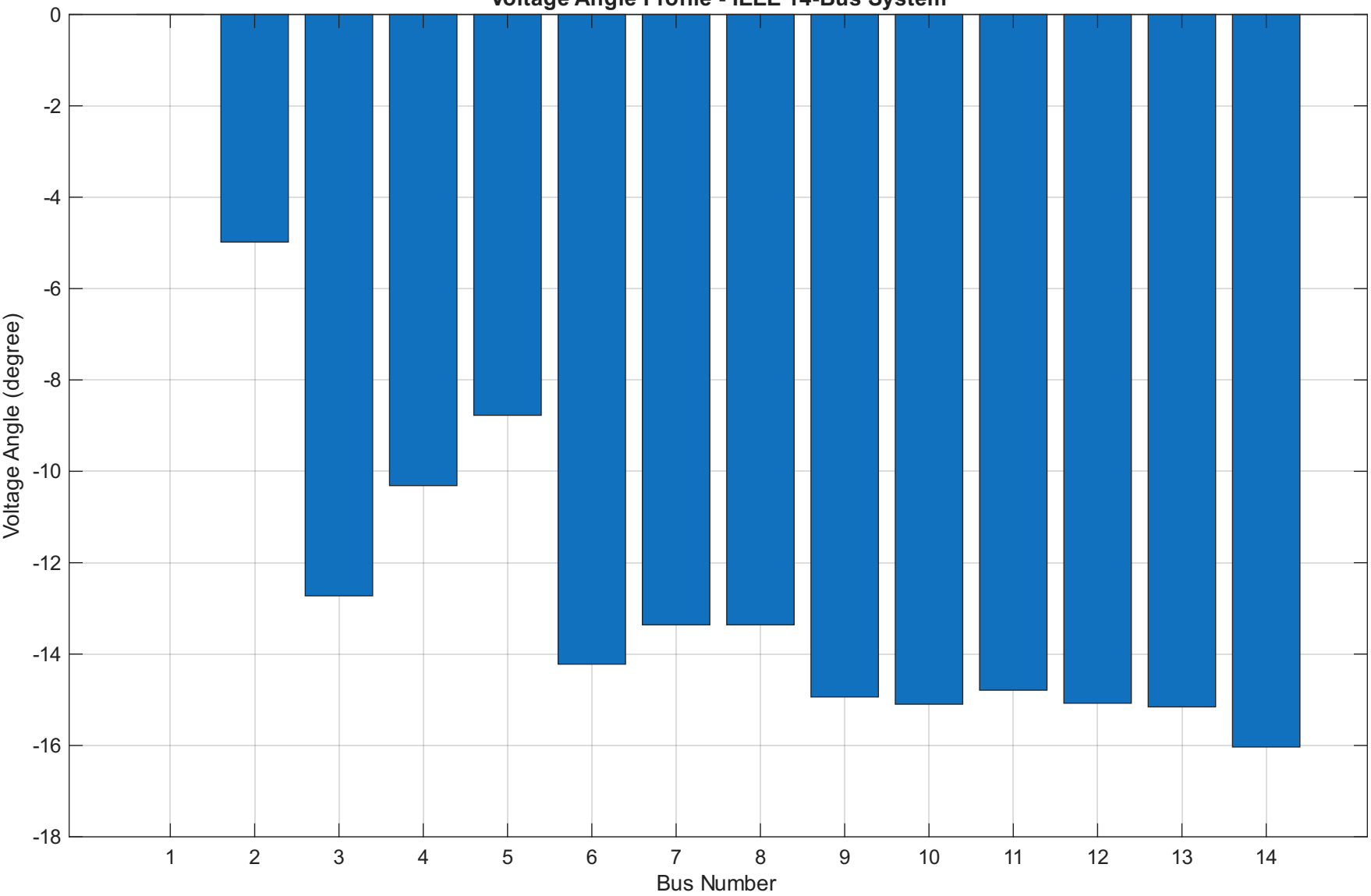
Voltage Angle Profile - IEEE 14-Bus System
