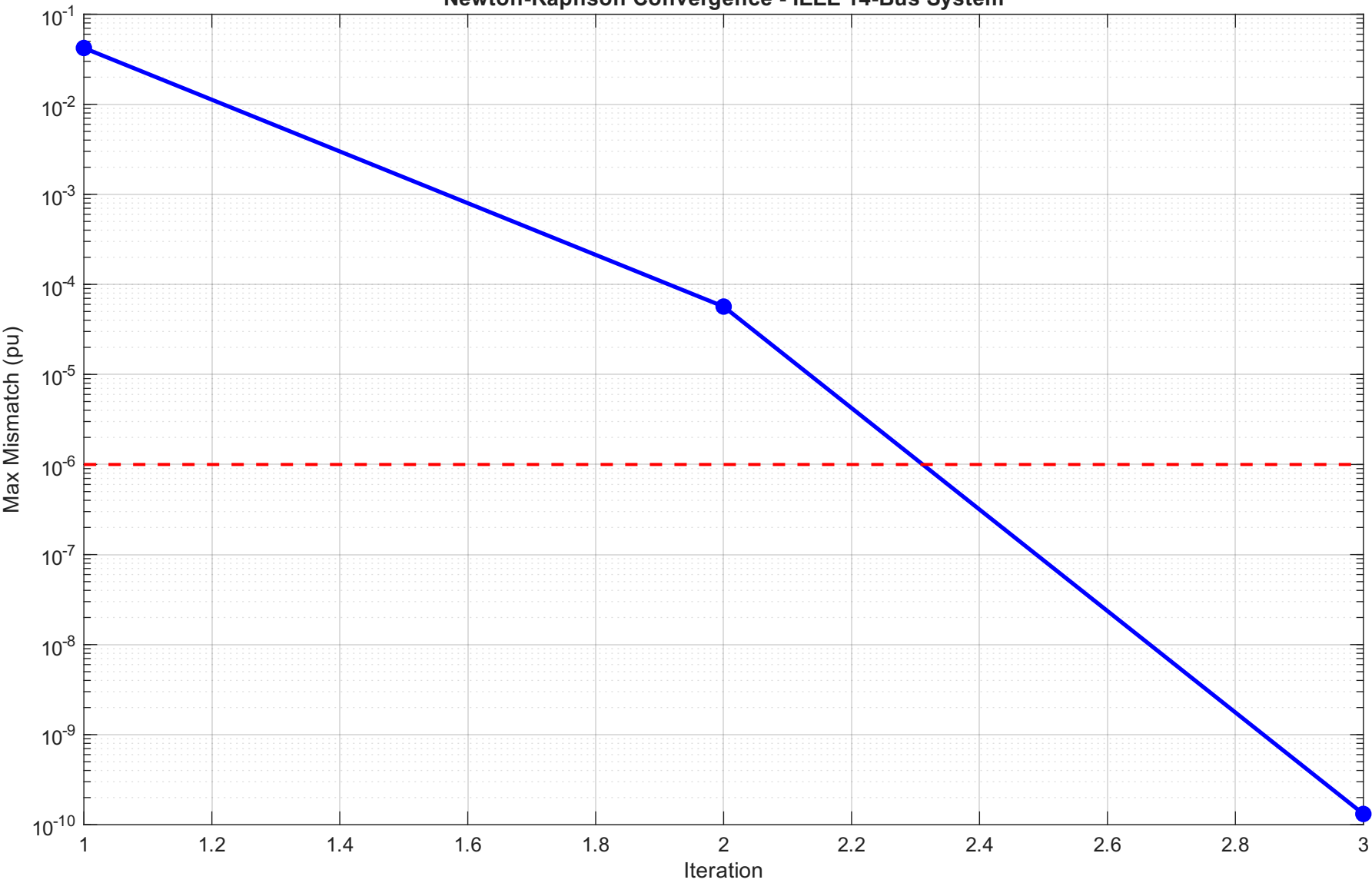
Newton-Raphson Convergence - IEEE 14-Bus System
