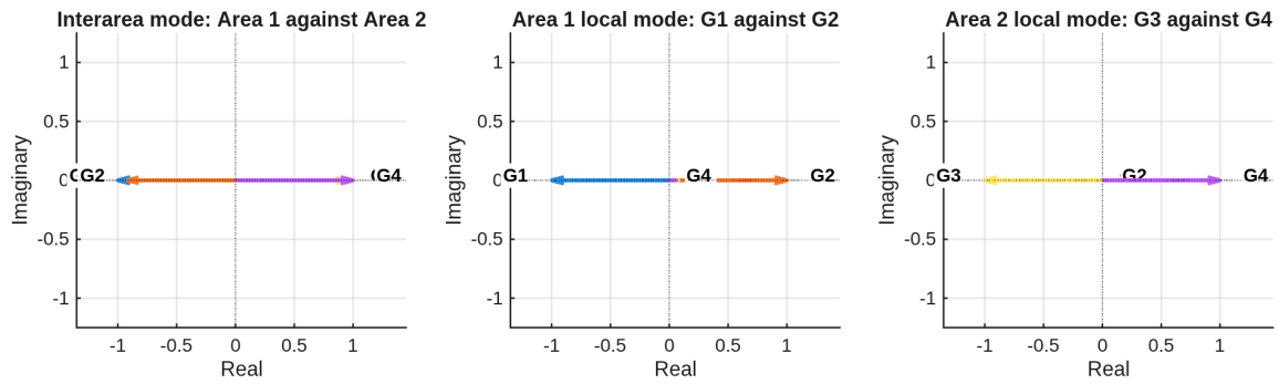
Figure 6: Rotor-speed mode shapes for the interarea and local rotor-angle modes under manual excitation.
