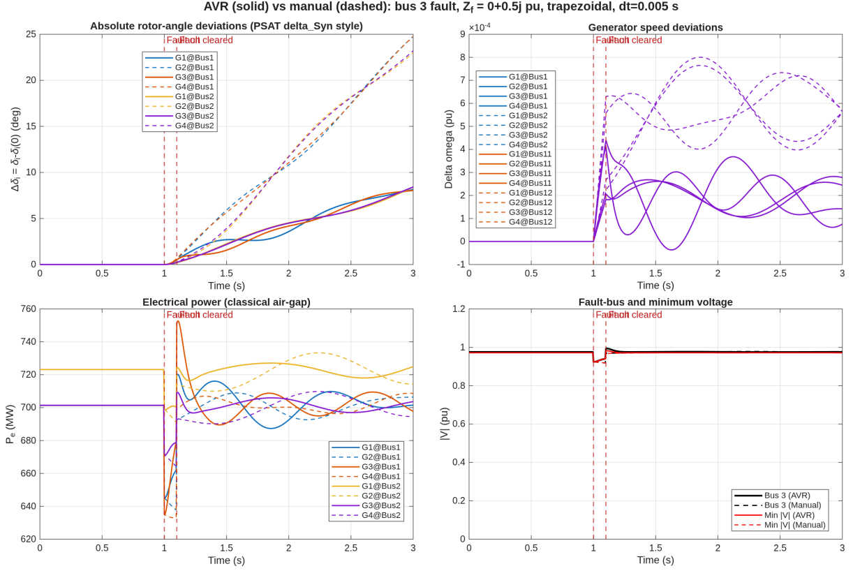
Figure 7: Special comparison: AVR (solid) versus manual excitation (dashed) for the same bus-3 fault. Each colour is one generator; solid curves use the five-state AVR model (the book’s configuration), dashed curves hold E_{fd} constant (16-state manual model). The curves expose the different rotor-angle, speed, power, and voltage responses under the identical disturbance. Quantitative modal damping is determined from (38) and Table 10, not inferred from visual appearance.
