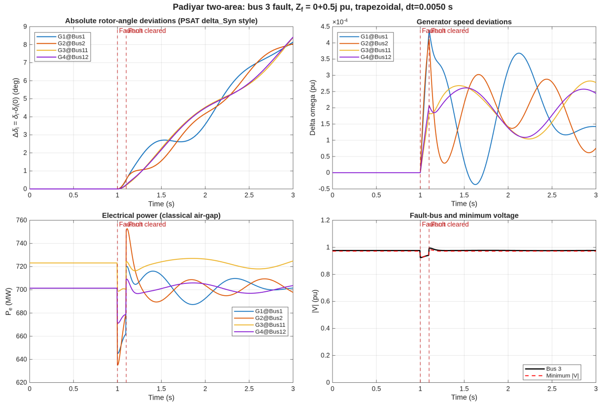
Figure 6: Bus-3 project fault response (AVR configuration, the book's 20-state model). Top-left: absolute rotor-angle deviations \delta_i(t) - \delta_i(0) (PSAT \delta_{Syn} style). Top-right: generator speed deviations. Bottom-left: air-gap electrical power. Bottom-right: fault-bus voltage and system minimum voltage. Red markers show fault application and clearance. This is the canonical 2 \times 2 TS display used by the in-house run_ts launcher; the manual-excitation comparison is reported numerically in Table 11 above.
