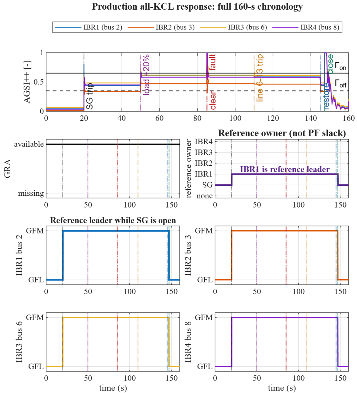
Figure 2: Bounded AGSI++, GRA, reference ownership, and separate IBR1–IBR4 mode timelines. The owner trace identifies IBR1 at bus 2 as the grid-forming angle/frequency leader while the SG is open. All IBRs are GFL before 20 s, GFM until the accepted handback, and GFL thereafter.
