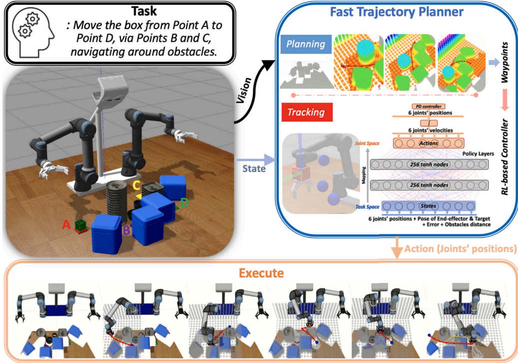
Fig. 1. System Overview: The Kinect sensor captures visual data to create an FSA-enhanced 3-dimensional (3D) map of the environment. This map is used with B-spline optimization to generate waypoints for kinodynamic path searching. These waypoints, along with the manipulator's state, inform the RL-based controller that adjusts the positions of the 6 joints of the manipulator.
