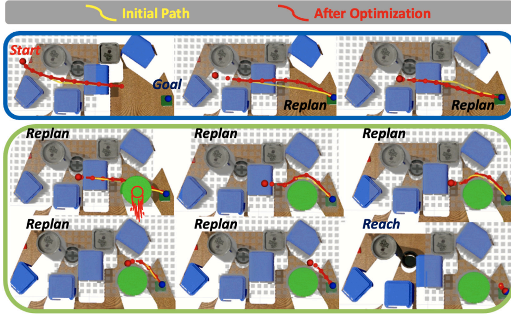
Fig. 3. Trajectory Planning Process: This example illustrates trajectory planning in a dynamic environment, where the yellow trajectory signifies initial planning. The start and target points are marked by a red and a blue ball, respectively. Upon encountering an unforeseen obstacle, represented by a green cylinder, the system triggers a replanning mechanism. Initially, the path does not circumvent the obstacle due to outdated map data. However, once the obstacle is detected, the system generates a new trajectory to navigate around it. This revised path, highlighted in red with waypoints, serves as input for the RL-based controller, ensuring adaptive and efficient navigation.
