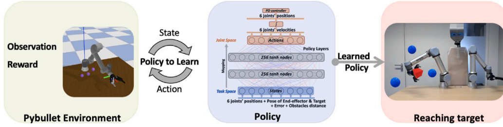
Fig. 6. Learning Strategy Deployment Overview: The agent is first trained in Pybullet to learn the task-to-joint space mapping of the UR5e manipulator. This trained policy is then adapted from one simulation to another (Sim-to-Sim) in Gazebo and applied directly to real-world robot scenarios without further fine-tuning.
