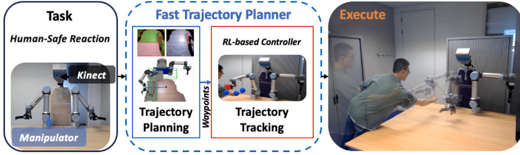
Fig. 7. Fast Trajectory Planner: This diagram illustrates the workflow of the fast trajectory planner, which combines real-time perception, B-spline-based trajectory optimization, and RL-based control. The system dynamically replans trajectories in response to changes, ensuring safe and efficient navigation during reactive tasks.
