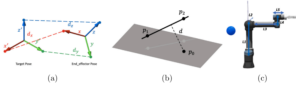
Fig. A.14. (a) The difference calculation between the end-effector and the target, integrating the sum of distance errors from three points defined along orthogonal axes. (b) Distance between a point and a space line. (c) d_{obs} is the obstacle (blue) to 5-link distance.
