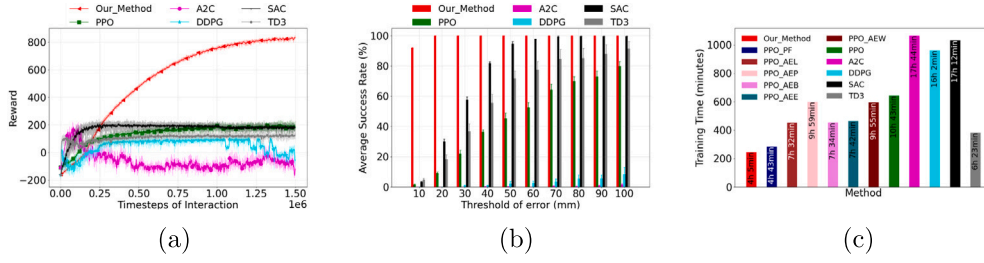
Fig. 9. Summary of Comparison Experiments: (a) Comparison result of accumulated reward utilizing 5 random seeds for our method and other baselines; (b) Comparison of success rate on reaching task with obstacles; (c) Comparison result of training time for different methods.
