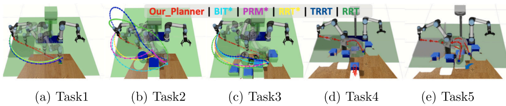
Fig. 12. Planner Comparison: Results from a single run for each planner across five tasks: Task 1 in an obstacle-free area; Task 2 with two additional obstacles; Task 3 in a cluttered scene; Task 4 featuring a moving obstacle near the goal; and Task 5 involving changing the goal as the end-effector nears it.
