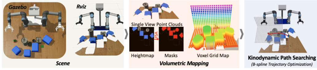
Fig. 2. Illustration of perception-aware Trajectory Planning: Using the FSA, object masks are merged with point clouds to create a Voxel Grid Map, providing a detailed basis for improved navigation and planning decisions.
