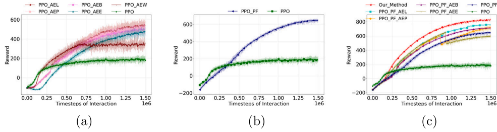
Fig. 8. Summary of Ablation Experiments: (a) Accumulated reward comparison for PPO with various AE methods across 5 random seeds; (b) PPO with PF method compared using 5 random seeds; (c) PPO performance with dual enhancements over 5 seeds. Variance is depicted by shaded areas.
