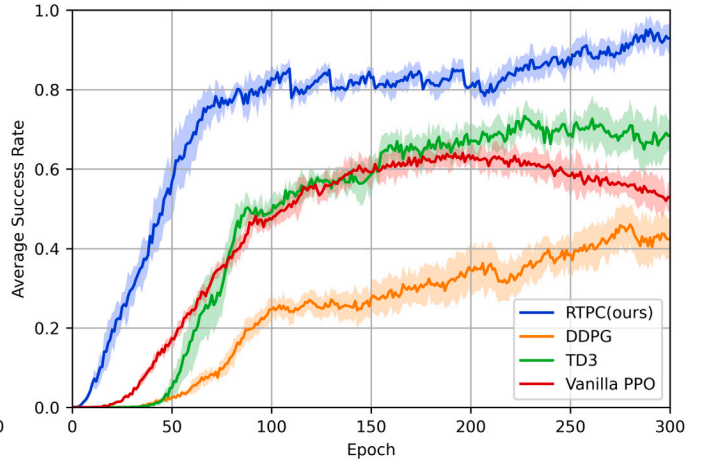
b) Success rate curves of different algorithms.
