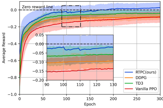
a) Training curves of different algorithms.
