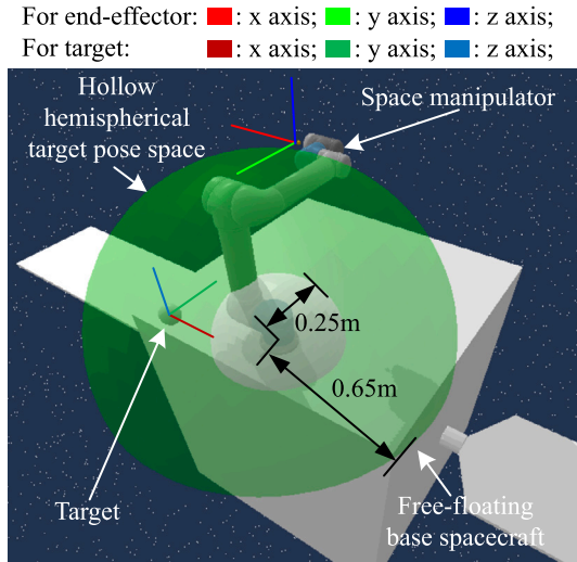
Fig. 5. Simulation environment of the free-floating space manipulator system.
