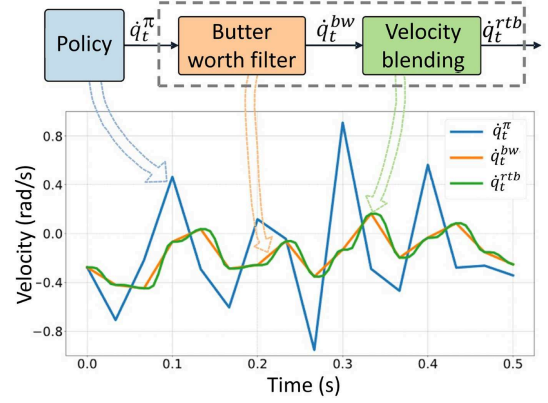
Fig. 4. An illustration of the RTB scheme.
