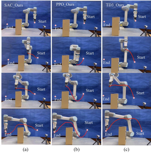
Fig. 6. Frame-by-frame plots under the safe reaching task with one obstacle using three different strategies: (a) SAC_Ours with the combination of BF and VB; (b) PPO_Ours with the combination of BF and VB; and (c) TD3_Ours with the combination of BF and VB.
