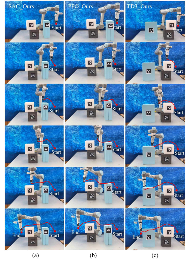
Fig. 8. Frame-by-frame plots under the safe reaching task with multiple obstacles using three different strategies: (a) SAC_Ours with the combination of BF and VB; (b) PPO_Ours with the combination of BF and VB; and (c) TD3_Ours with the combination of BF and VB.
