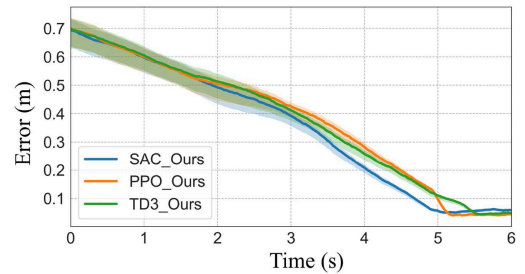
Fig. 9. Real-time tracking errors of the end-effector under the safe reaching task with multiple obstacles using three different strategies.
