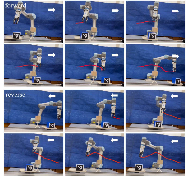
Fig. 12. Frame-by-frame plots under the 1-D dynamic target tracking task using our proposed approach.
