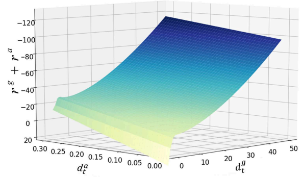
Fig. 3. Variations of the reward function as the robot approaches the target.
