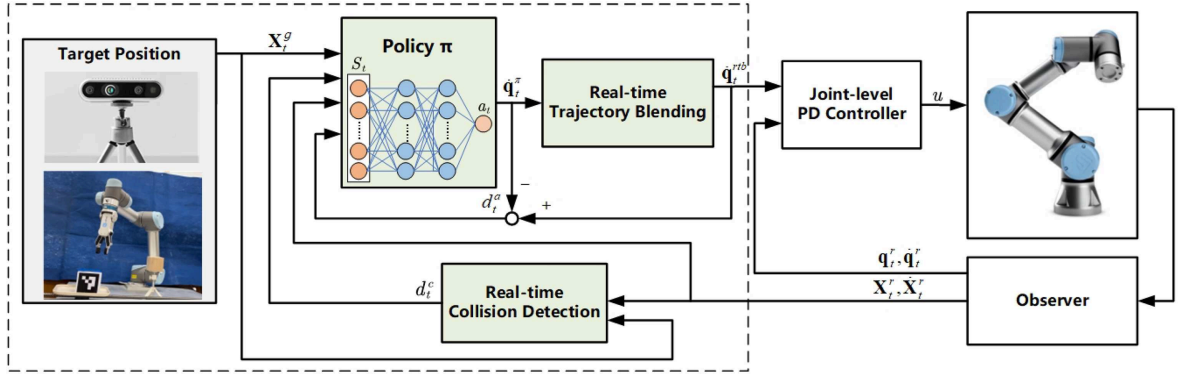
Fig. 2. An overview of the proposed RL-based visual servoing control architecture. X_t^g represent the target pose, X_t^r and \dot{X}_t^r denote the end-effector pose and velocity, respectively, q_t^r and \dot{q}_t^r denote the joint position and velocity, respectively, q_t^\pi is the policy output and q_t^{rtb} is the reference joint velocity generated by the RTB process, u denotes the control signal, d_t^a is the prefetched safe distance generated by the RTB module, and d_t^c is the actual safe distance.
