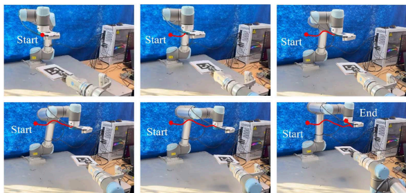
Fig. 14. Frame-by-frame plots under the 2-D dynamic target tracking task using the proposed approach.
