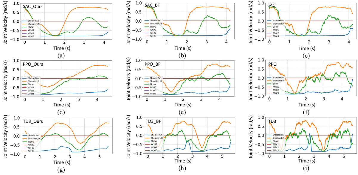
Fig. 10. Comparative analysis of robot joint velocity profiles with different strategies: (a)–(c) depict the joint velocity profiles using three different combinations of SAC; (d)–(f) depict the joint velocity profiles using three different combinations of PPO; and (g)–(i) depict the joint velocity profiles using three different combinations of TD3.
