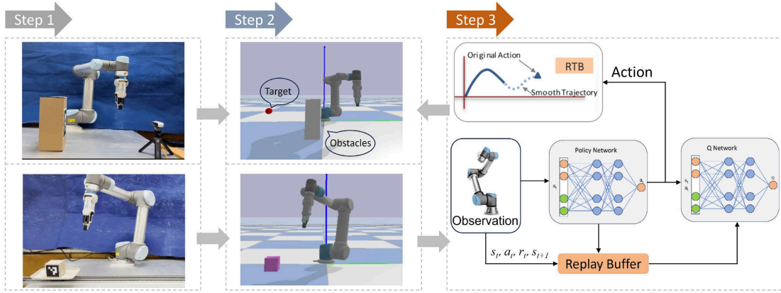
Fig. 1. An illustration of the proposed design procedure. In step 1, a real-world robot manipulator is constructed for motion trajectories collection and experimental verification. In step 2, building a digital twin environment for RL training with RCD. In step 3, training the RL policy with RTB by utilizing the location of obstacles as an observed state.
