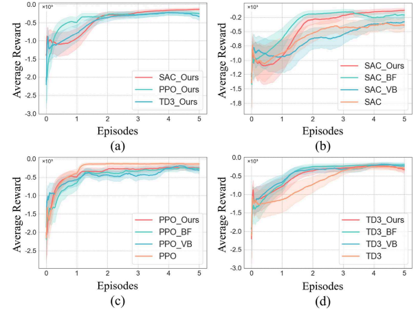
Fig. 5. Average rewards during the training process with different strategies: (a) SAC_Ours, PPO_Ours, and TD3_Ours with the combination of BF and VB; (b) different SAC strategies with or without BF and VB; (c) different PPO strategies with or without BF and VB; and (d) different TD3 strategies with or without BF and VB.
