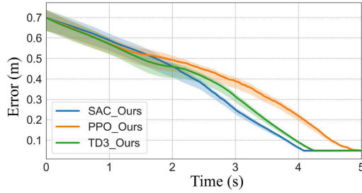
Fig. 7. Real-time tracking errors of the end-effector under the safe reaching task with one obstacle using three different strategies.
