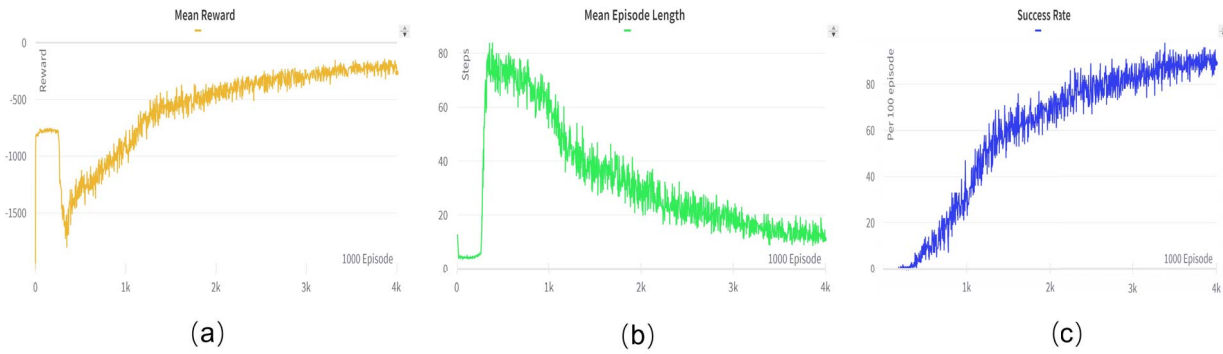
Figure 7. Model validation mean results for 100 episodes (a) Mean reward; (b) Mean episode length; (c) Success rate.
