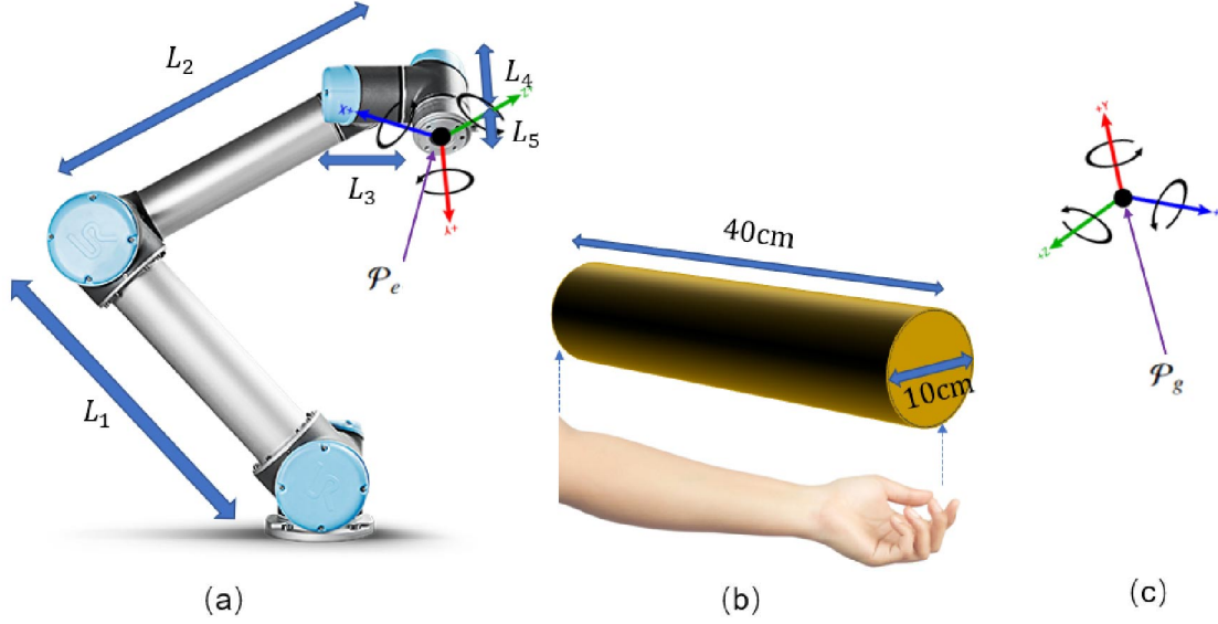
Figure 2. Graph illustration of the robot, moving obstacle and target (a) Robot links that may collide with other objects and the end-effector pose; (b) human forearm and hand modelled as a cylindrical obstacle (c) Target pose.
