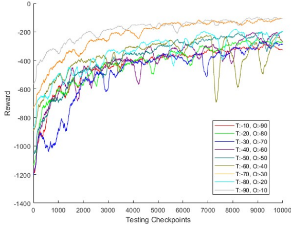
Figure 5. Nine reward curves for different combinations of positional and rotational reward weight.
