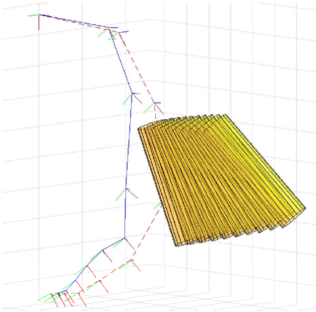
Figure 8. The robot end-effector trajectory obtained from two models on the same testing case. Yellow: The moving trajectory of the obstacle. Blue: The waypoints generated by the model trained with moving obstacles. Red: The waypoints generated by the model trained without obstacles.
