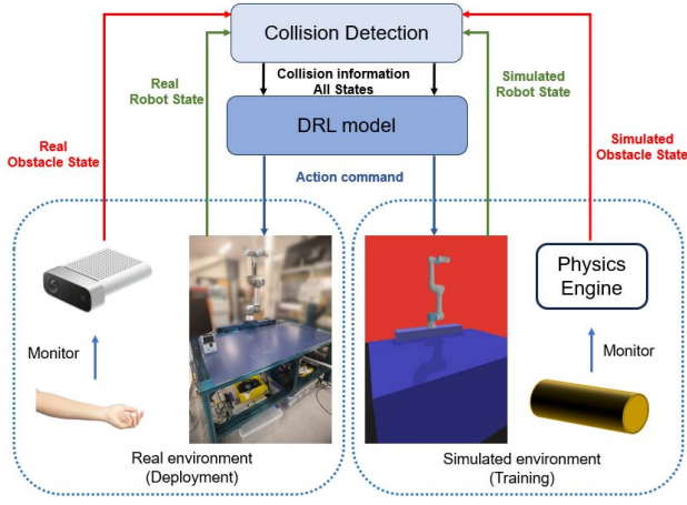
Figure 4. The framework for training and deploying the DRL model, minimises the reality gap.
