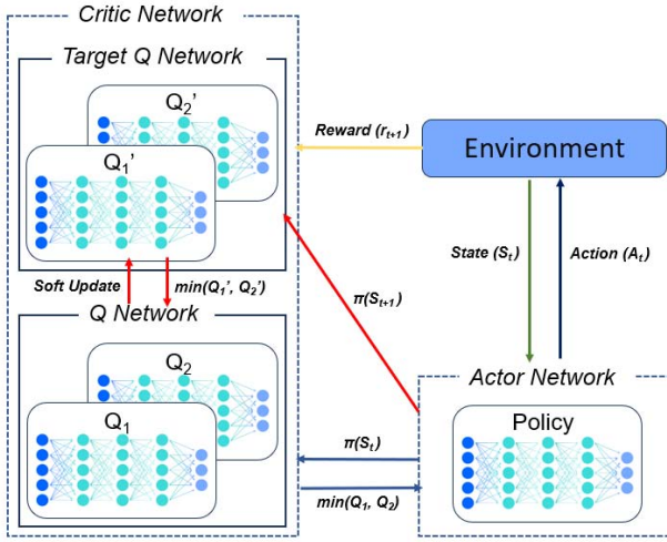
Figure 3. The network and environment interaction structure of the SAC algorithm
