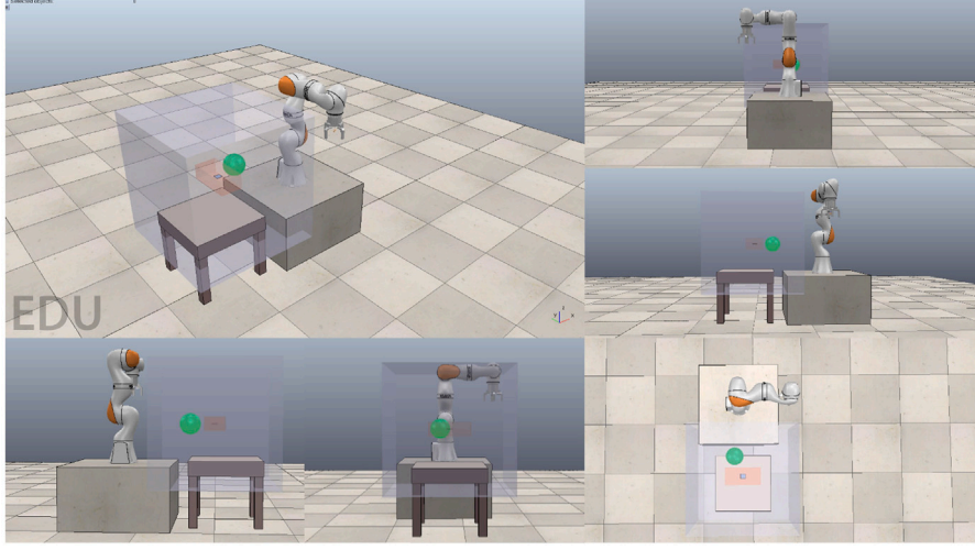
Fig. 6. Adaptive motion planning simulation environment for a robotic manipulator in a dynamic environment based on CoppeliaSim.
