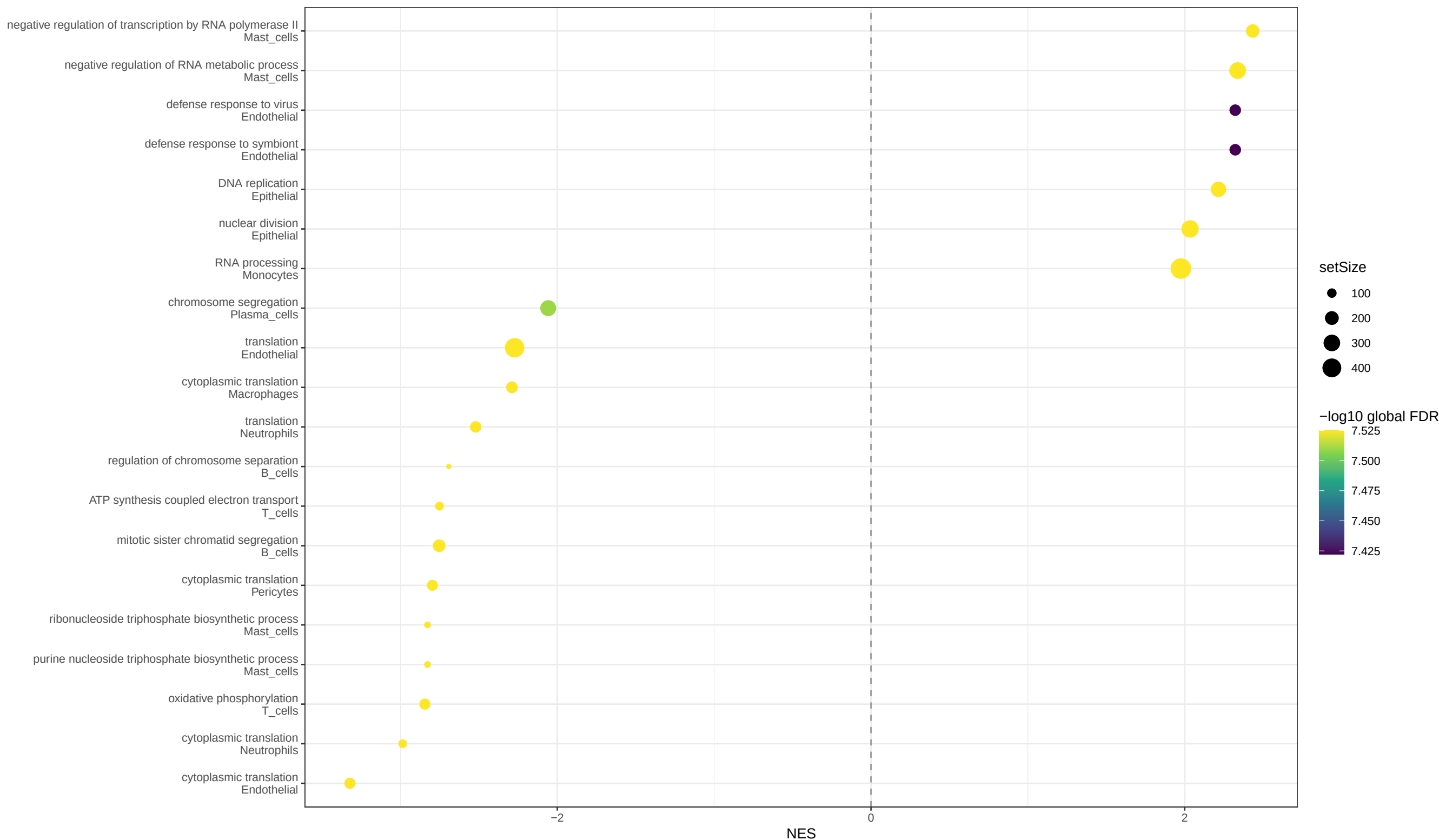
Exploratory ranked GO GSEA | top terms NES > 0: right-sided; NES < 0: left-sided | gene-set test, not independent validation
