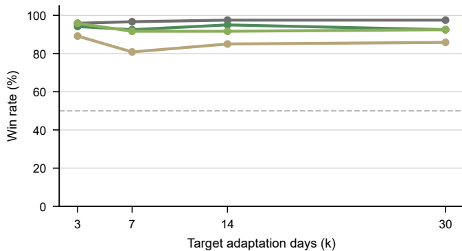
PA-MSR paired wins
