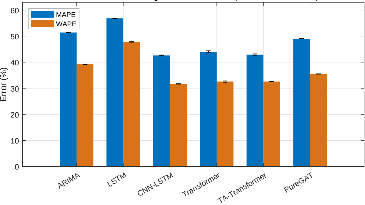
Cluster-level forecasting error on UMass-33 (3 seeds, mean \pm std)
