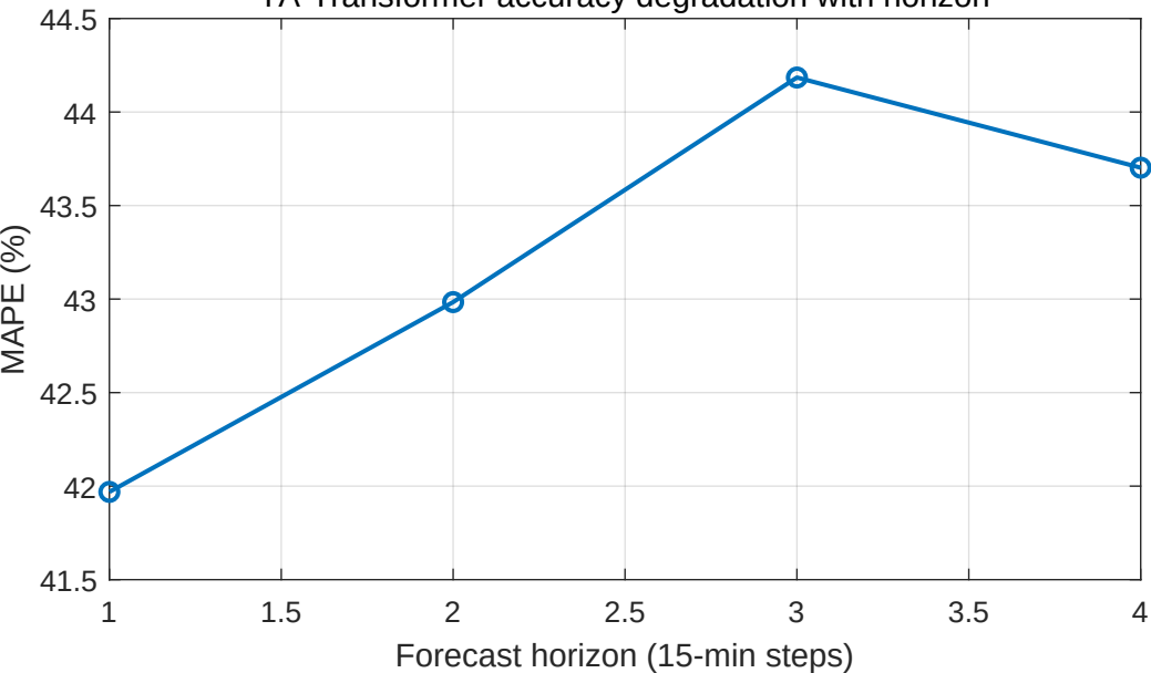
TA-Transformer accuracy degradation with horizon
