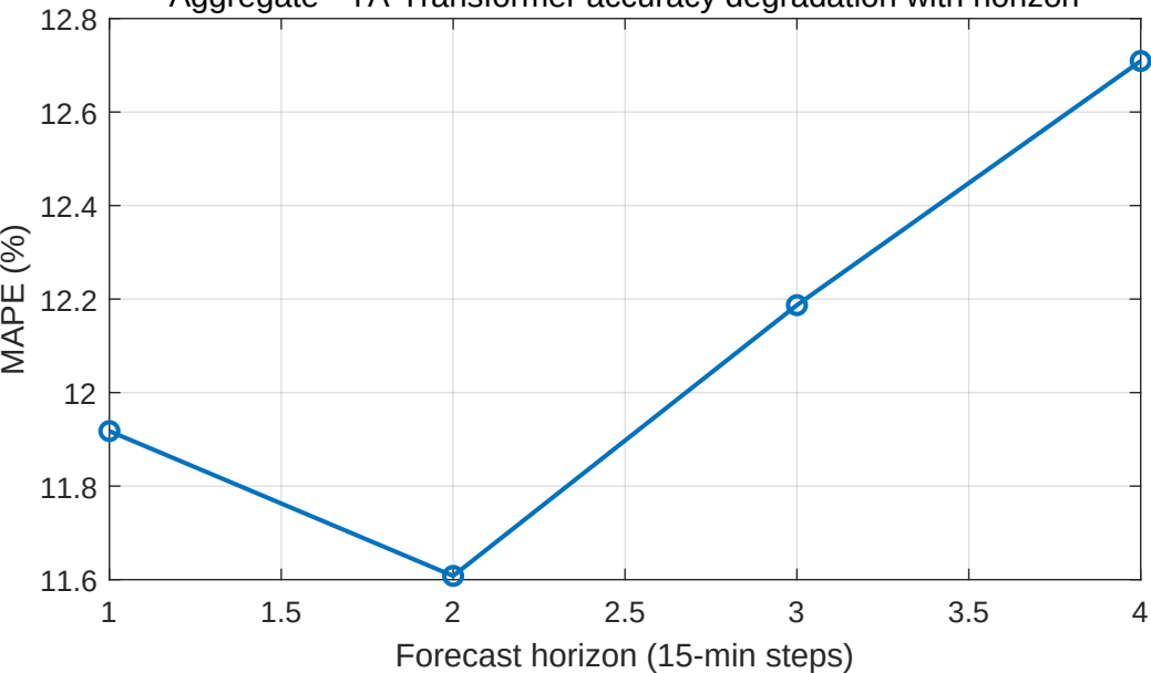
Aggregate - TA-Transformer accuracy degradation with horizon
