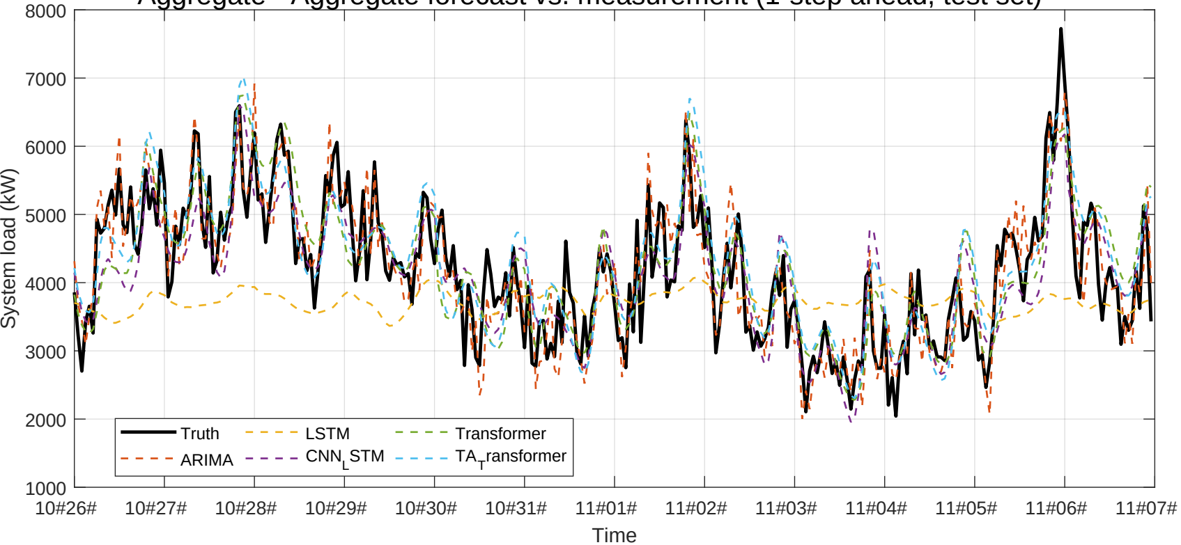
Aggregate - Aggregate forecast vs. measurement (1-step ahead, test set)
