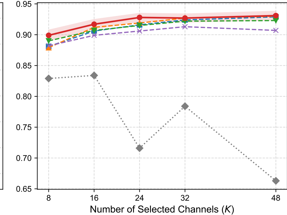
F1-score
