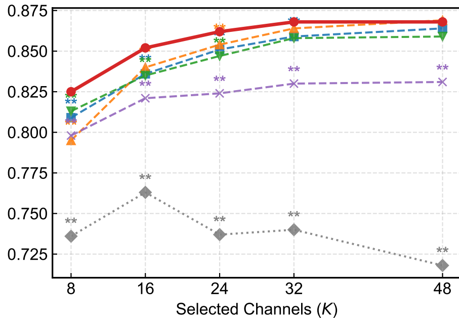
Balanced Accuracy
