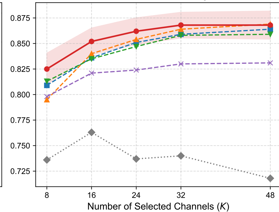
Balanced Accuracy
