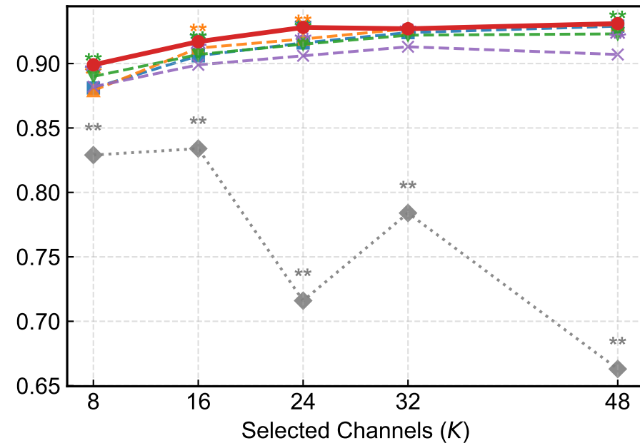
F1-score
