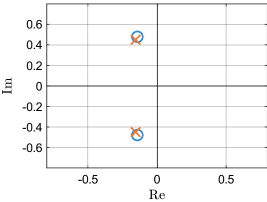
aerosonde — phugoid zoom
