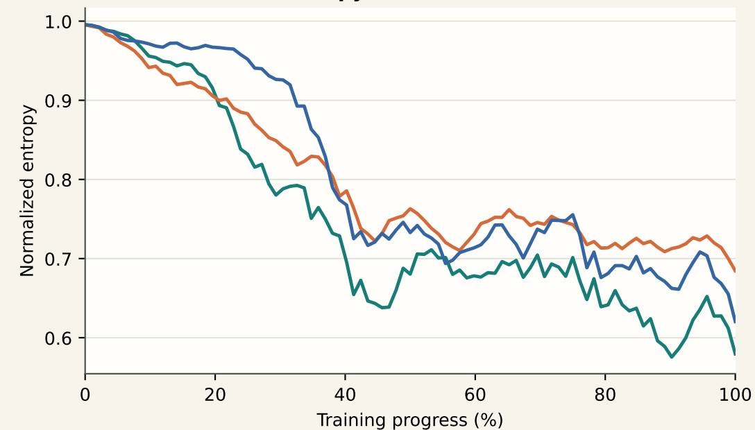
Visual attention entropy
