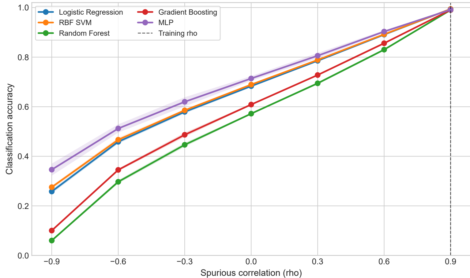
Distribution Shift with All Features
