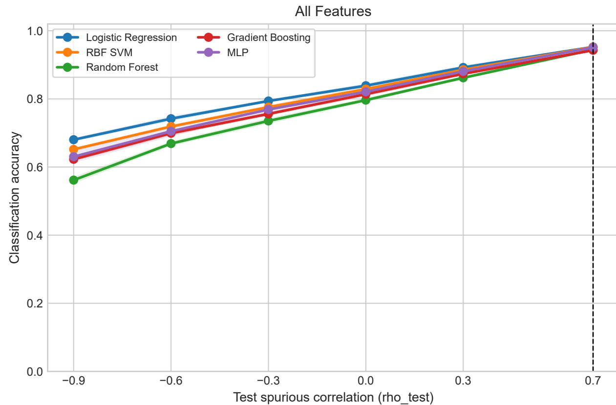
EXP-002 Shift Degradation — \rho_{\text{train}} = 0.7
