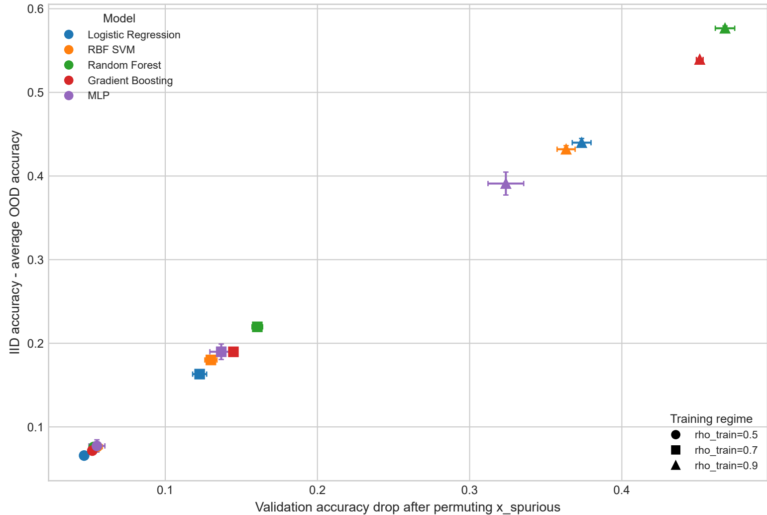
Spurious Reliance vs OOD Degradation
