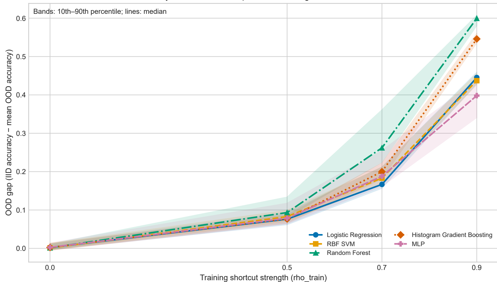
Family robustness envelopes across configurations and seeds
