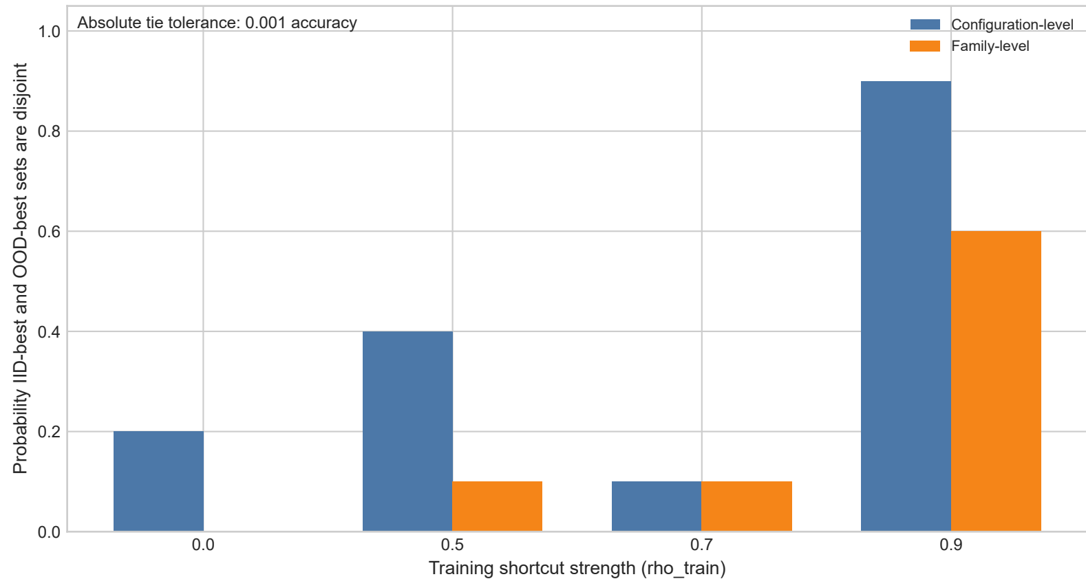
Tie-aware IID/OOD ranking reversal across 10 paired seeds
