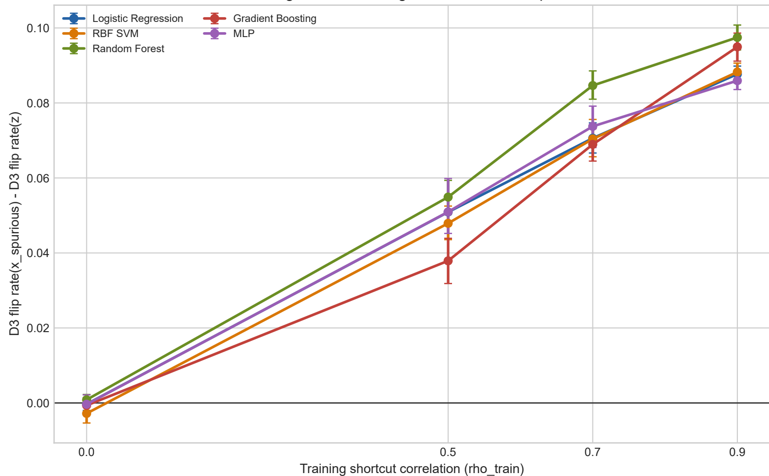
Training Shortcut Strength vs D3 Excess Flip Rate
