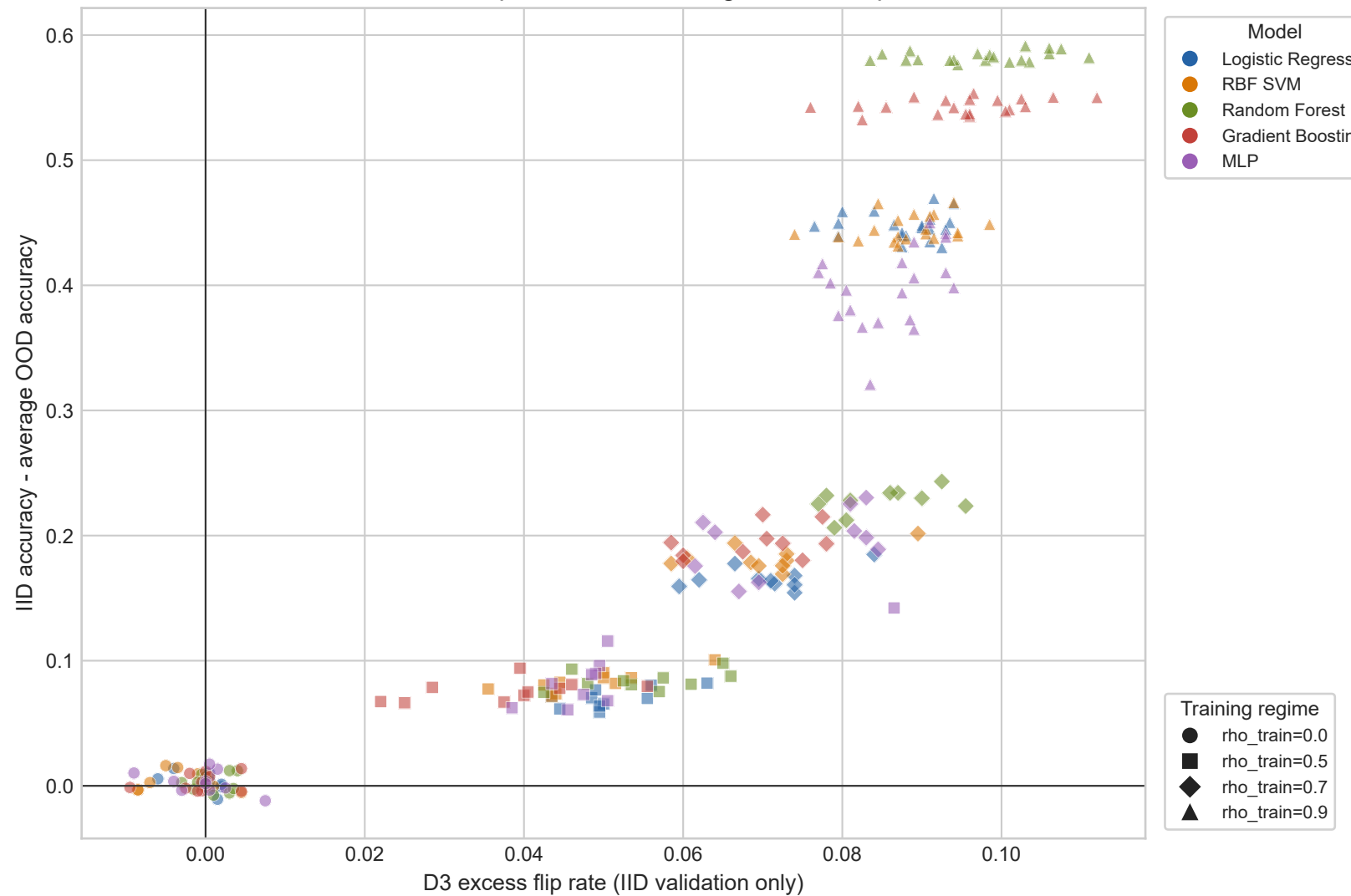
D3 Excess Flip Rate vs OOD Degradation Gap
