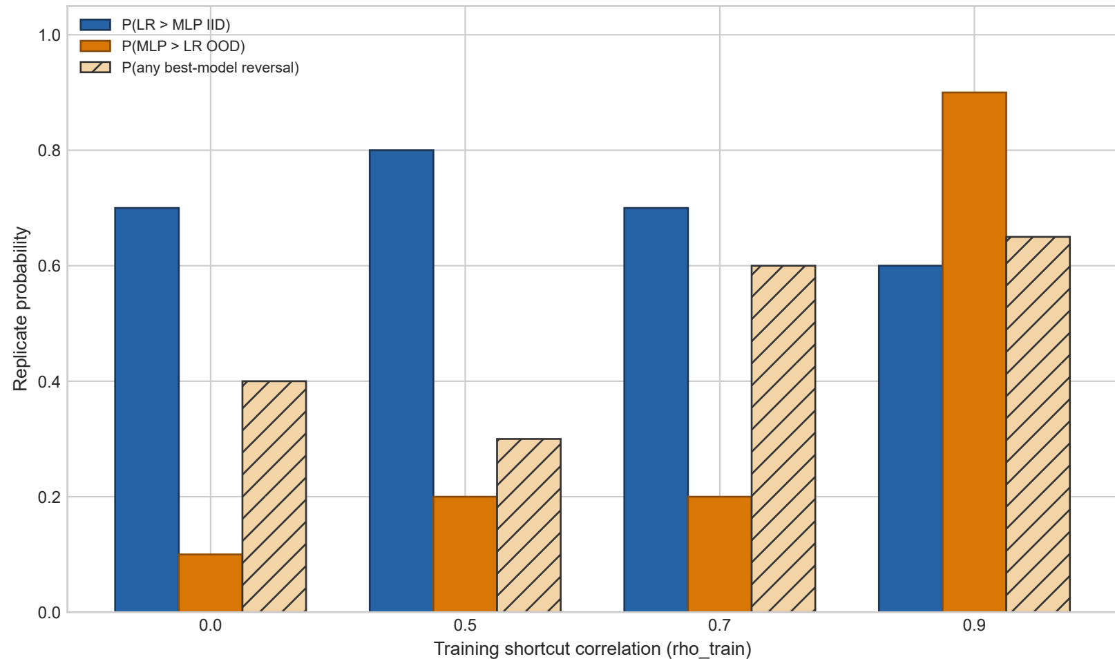
LR vs MLP Ordering and Best-Model Reversal Probability
