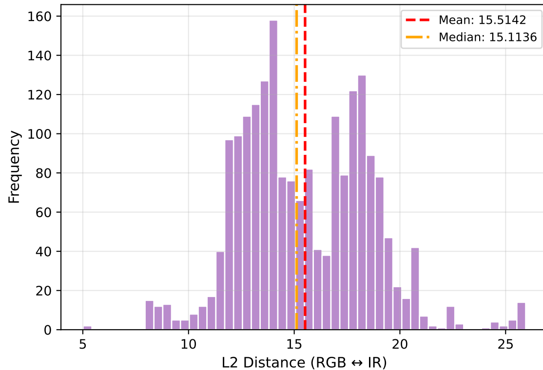
(b) Cross-Modal Distance Distribution (Lower = Better Alignment)
