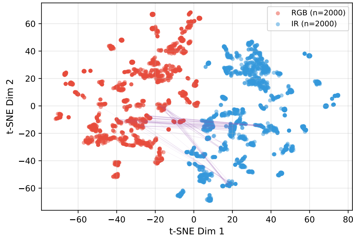
(a) RGB-IR Latent Space Distribution (with modality pairing lines)
