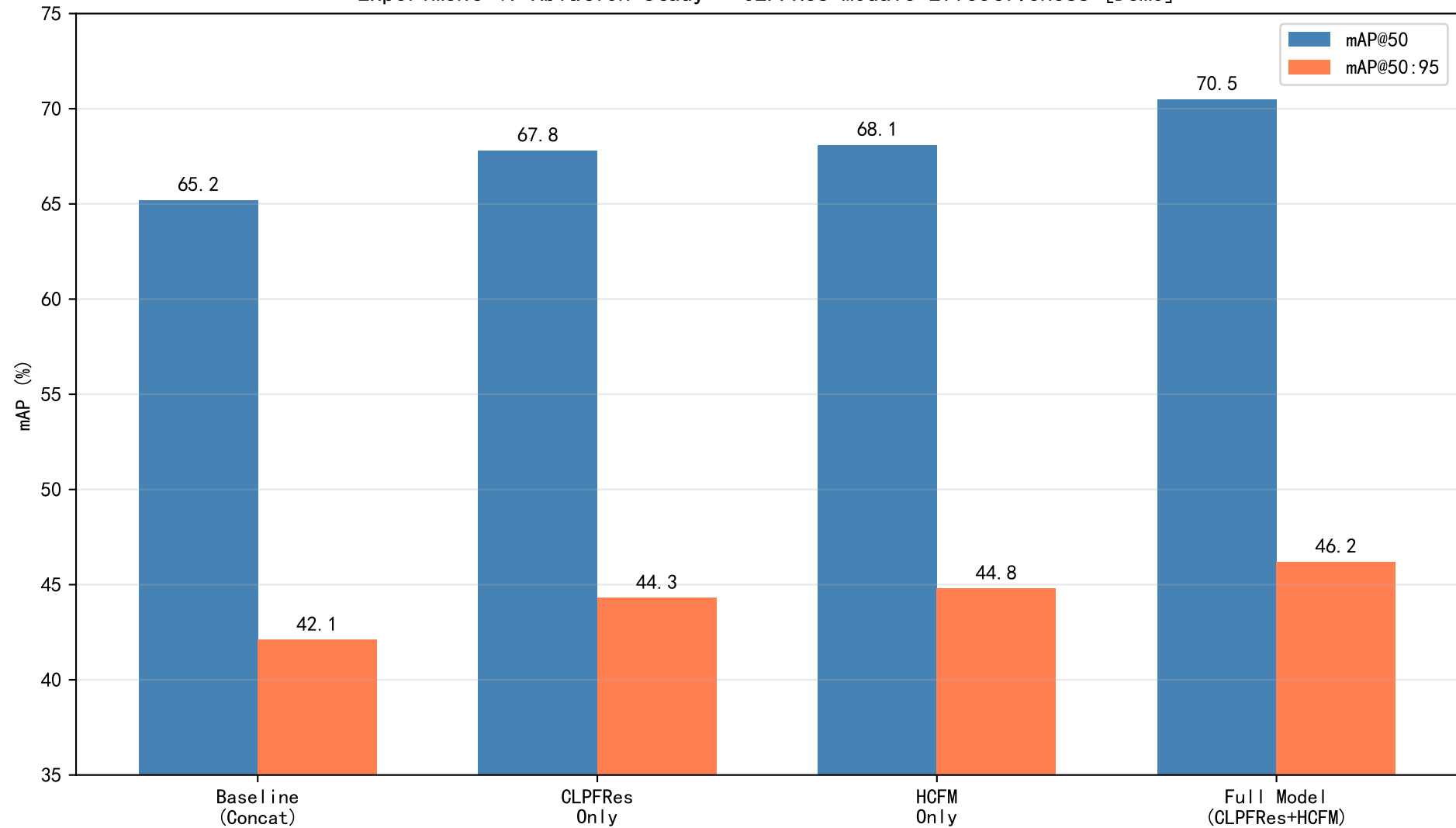
Experiment 4: Ablation Study - CLPFRes Module Effectiveness [Demo]
