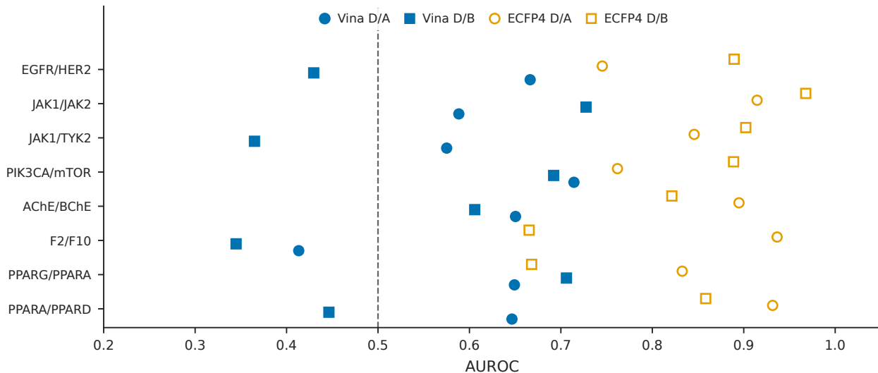
Vina rank AUROC and ECFP4 scaffold GroupKFold
