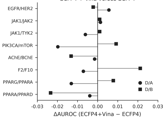
ECFP4 + Vina versus ECFP4
