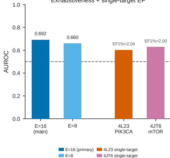
Exhaustiveness + single-target EF
