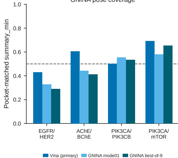
GNINA pose coverage
