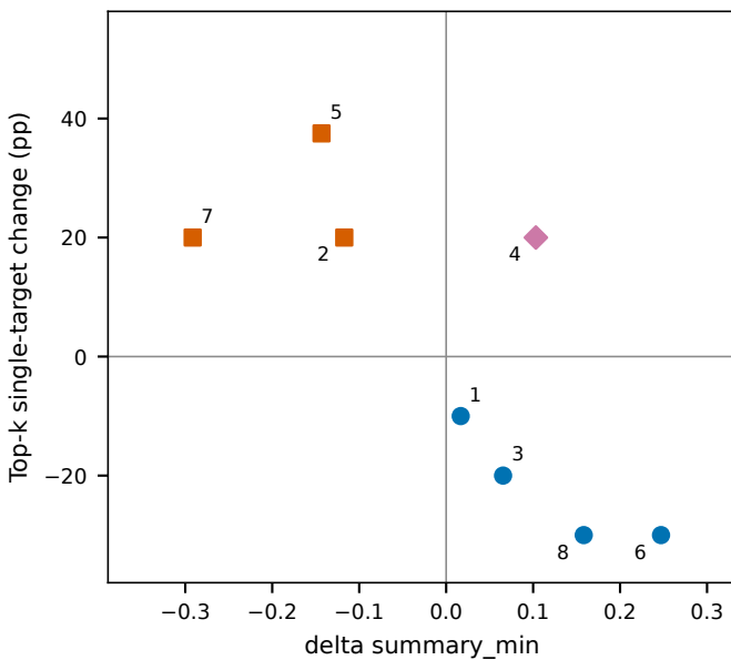
M2 vs M0
