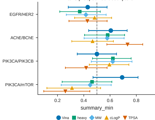
Vina vs prespecified descriptors
