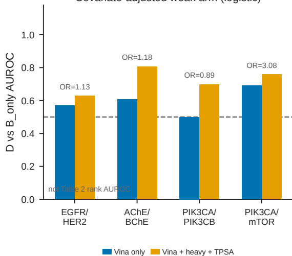
Covariate-adjusted weak arm (logistic)
