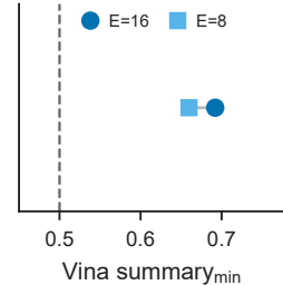
Search exhaustiveness
