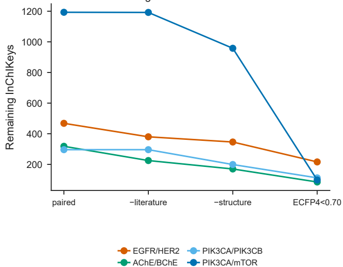
BindingDB-native filter cascade
