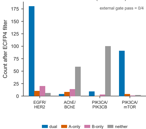
Four-state remainder (not docked)
