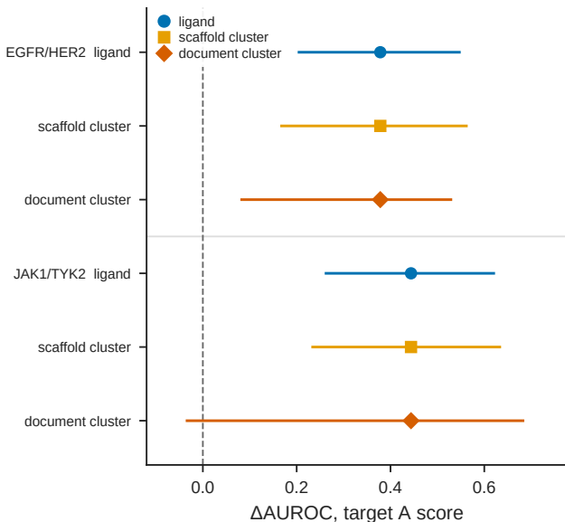
Resampling of flagship differences
