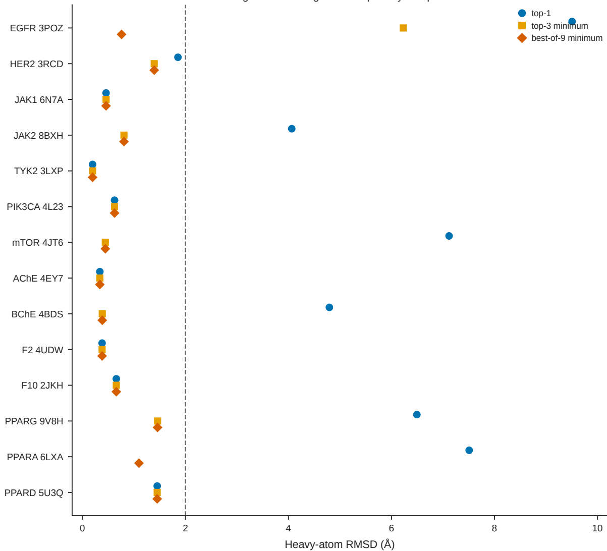
Cognate redocking of the 14 primary receptors
