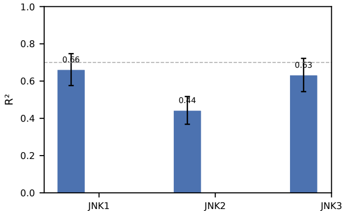
5-fold scaffold CV (mean \pm SD)
