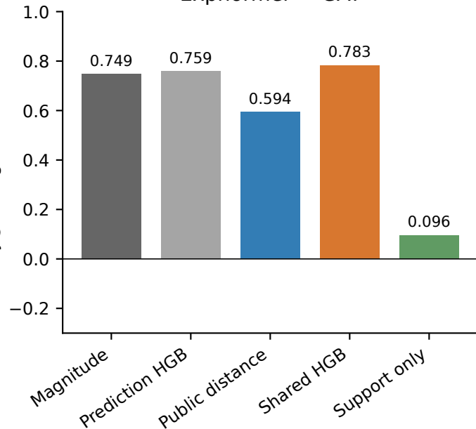
Exphormer → GAT
