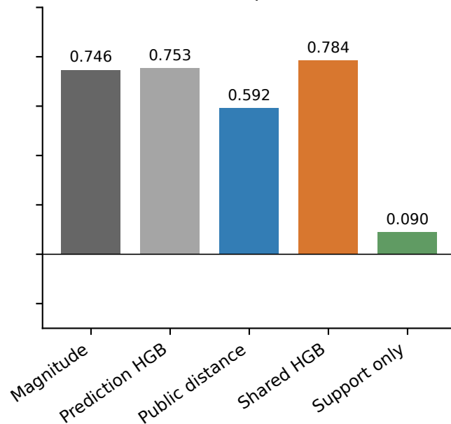
GAT → Exphormer
