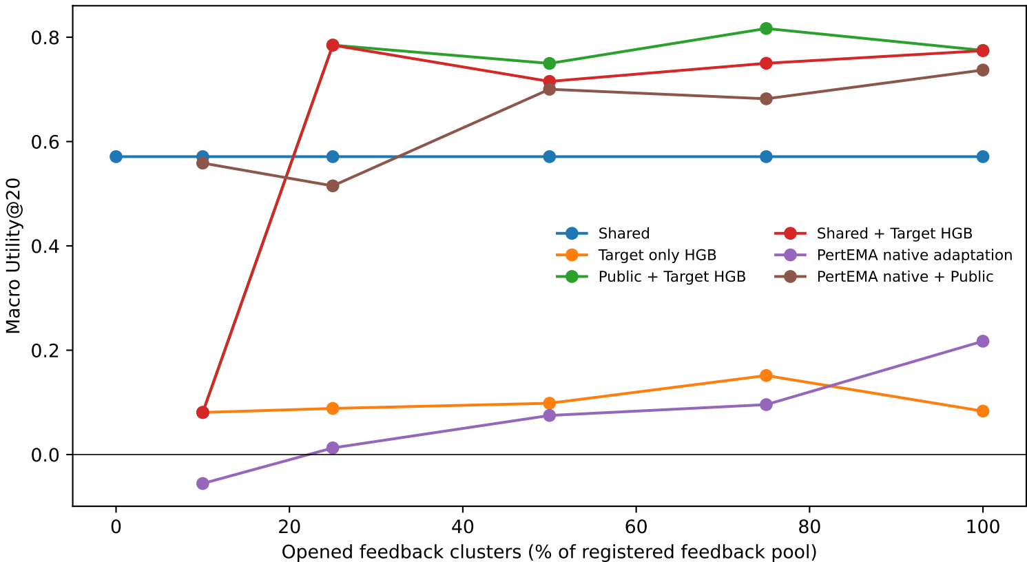
Common-axis feedback: same 212 holdout tasks
