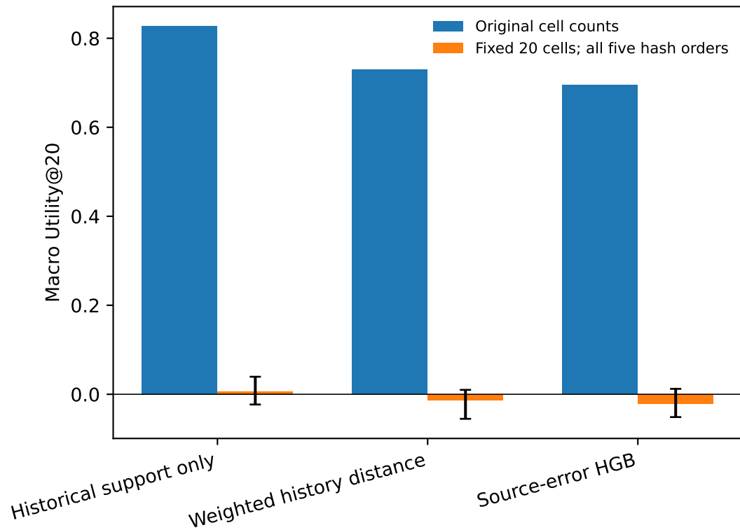
B. Fixed-size truth sensitivity (diagnostic)
