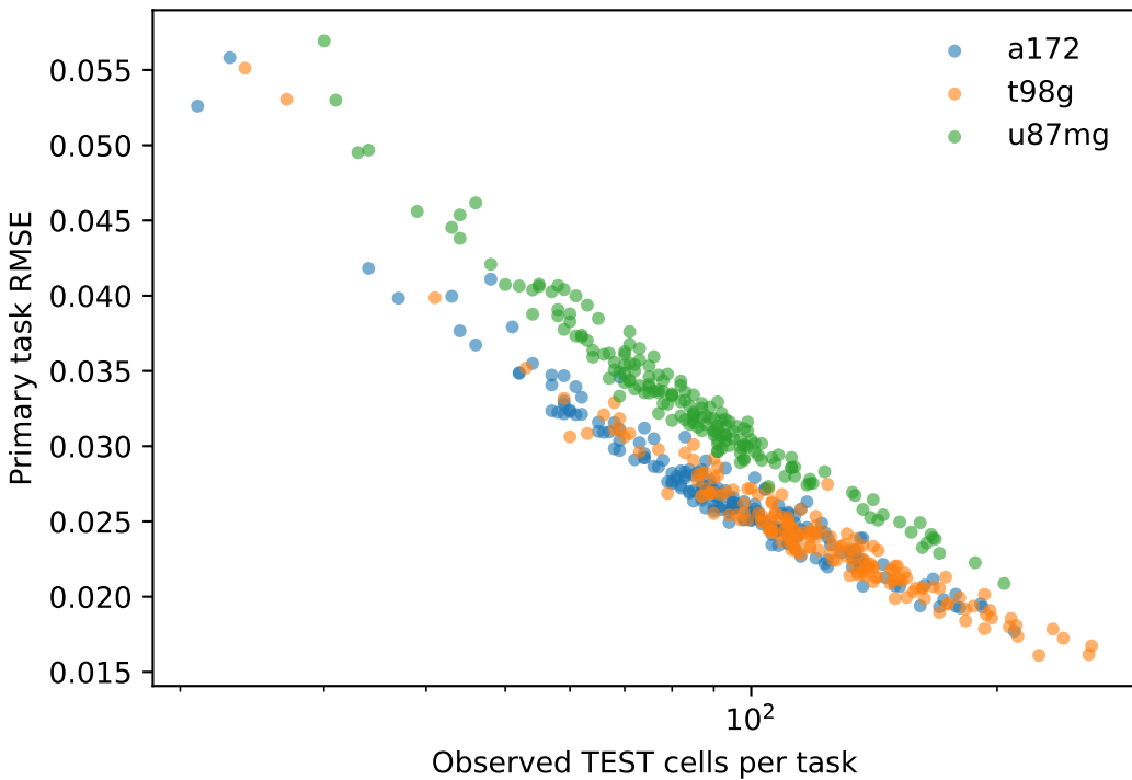
A. Observed error depends on sampling size
