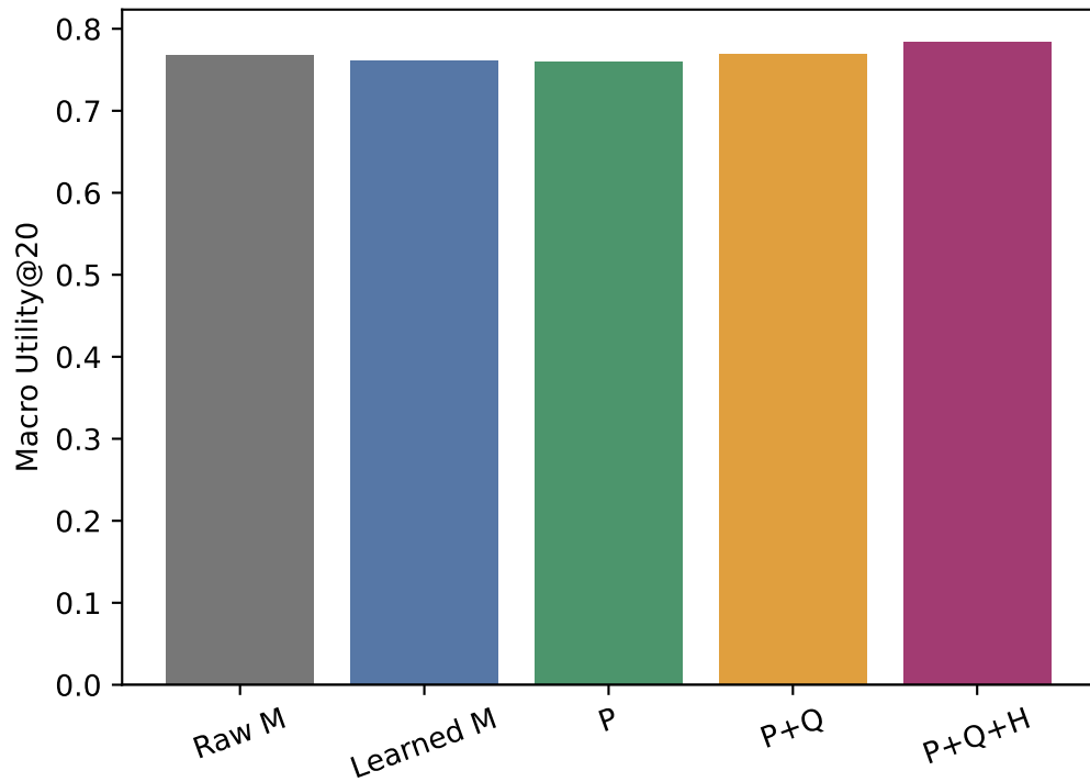
TxPert risk-information staircase (Ridge)
