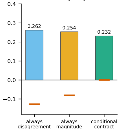
c Why a contract, not a fixed score (mean vs worst setting across 9 frozen settings; illustrative — prospective test = E201, sealed)
