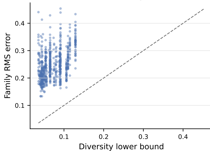
B Certificate tightness
