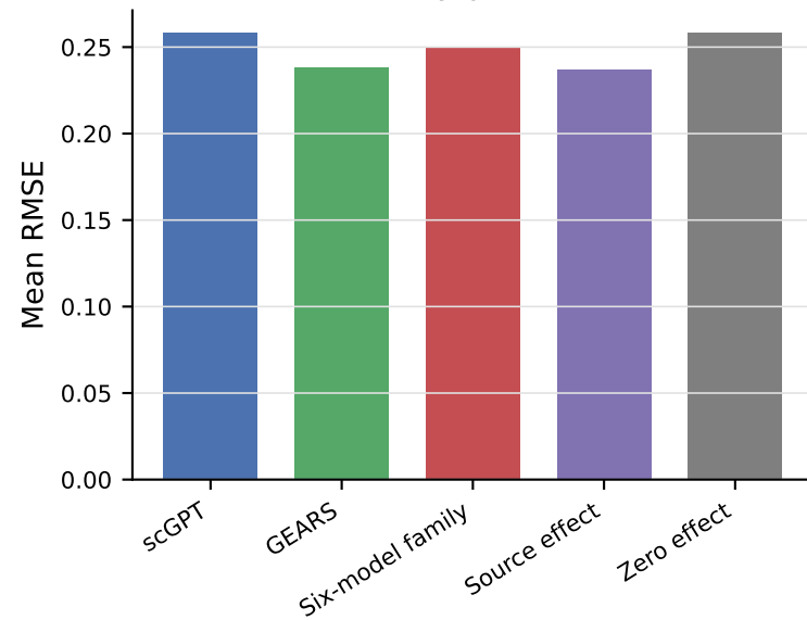
A Cross-study prediction error
