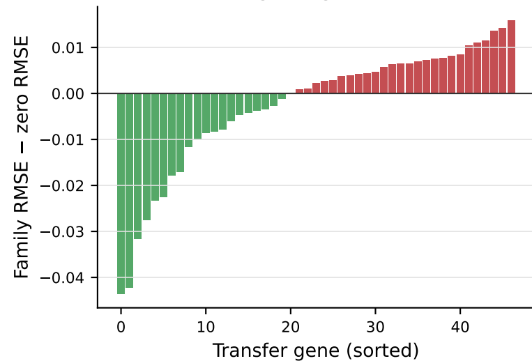
C Per-gene gain or loss
